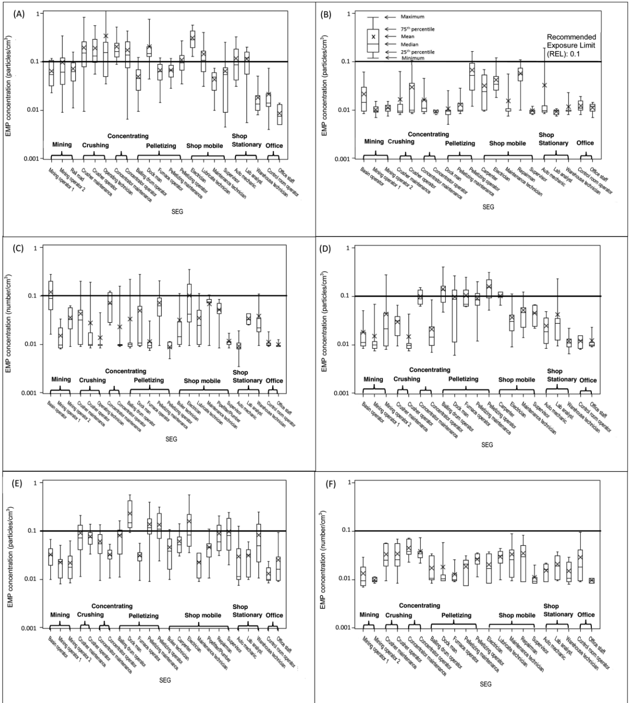
Supplement1. Box plot of total EMP for each SEG in mines A–F (the horizontal line indicates the NIOSH REL for EMP = 0.1 particles \text{cm}^{-3} ) 1 . Mine A in eastern zone. Mines B-F in western zone.
